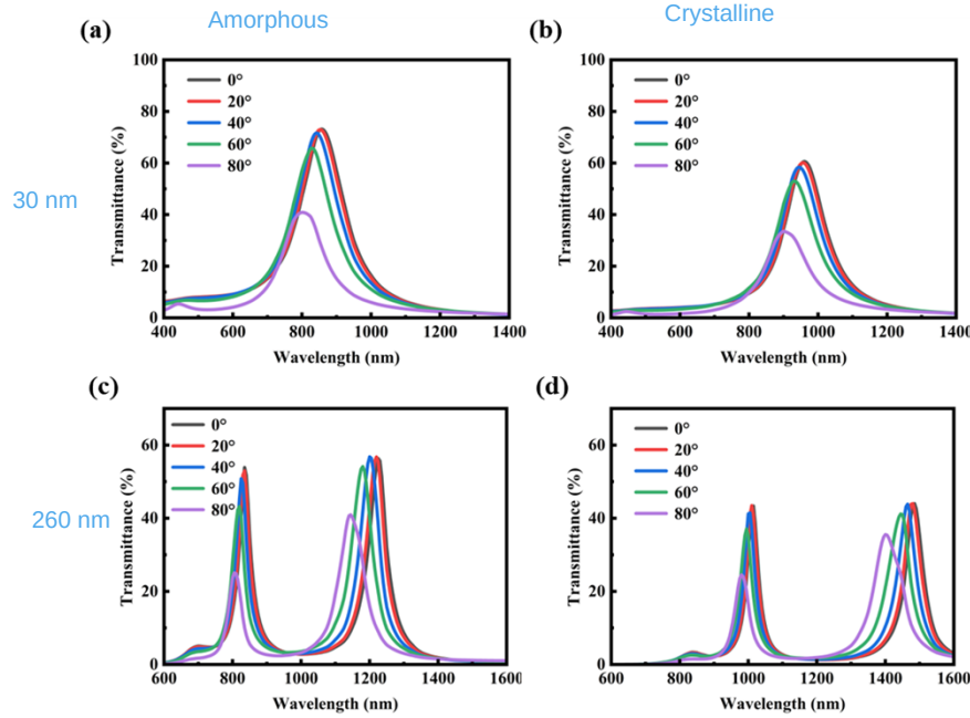
Fig. 4. The simulation transmission spectra of the multilayer film under different incident angles for \text{Sb}_2\text{Se}_3 thicknesses of 30 nm and 260 nm: (a) amorphous and (b) crystalline states at 30 nm; (c) amorphous and (d) crystalline states at 260 nm.
